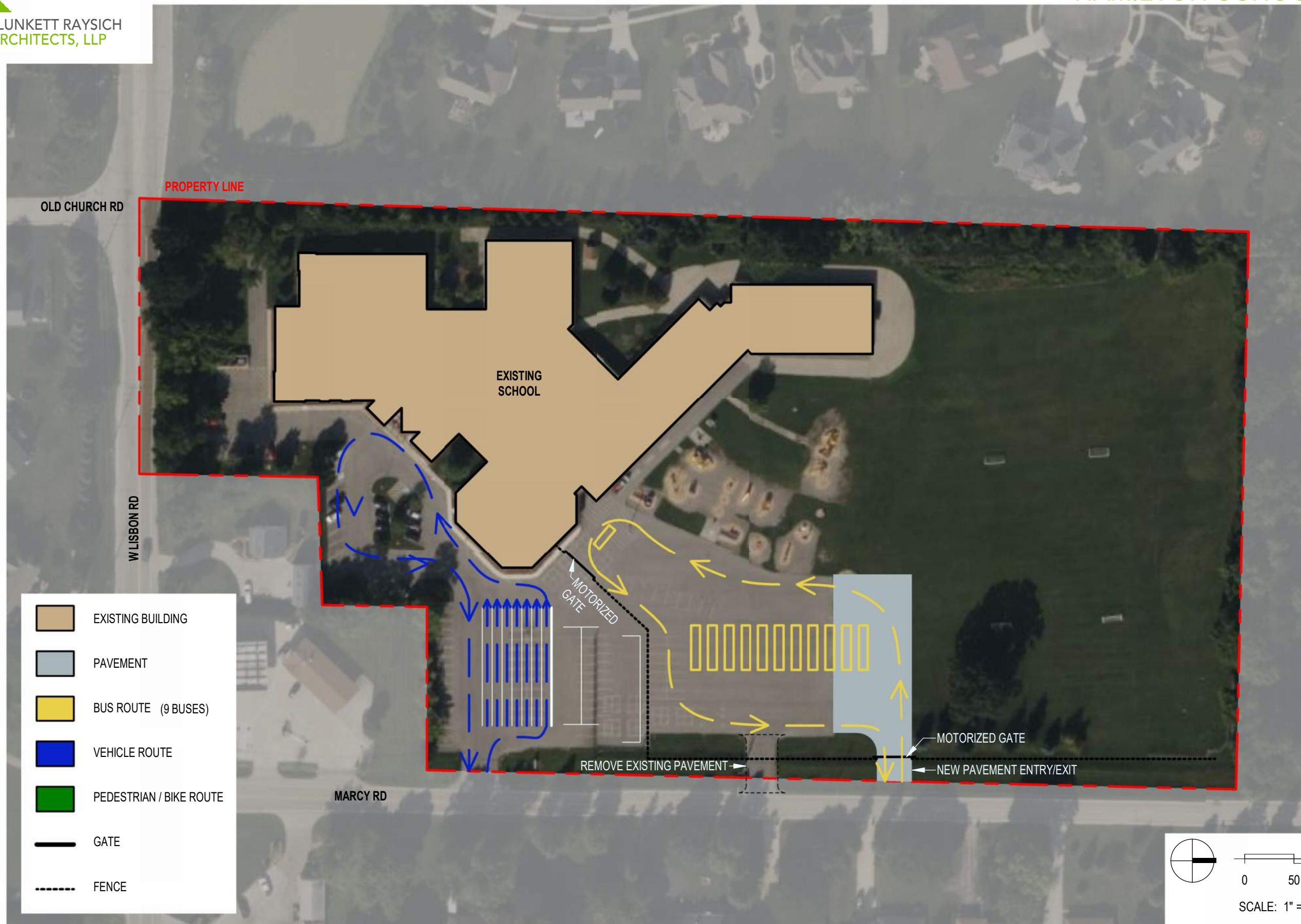
SITE PLAN - MARCY ES - PROPOSED OPTION 2
